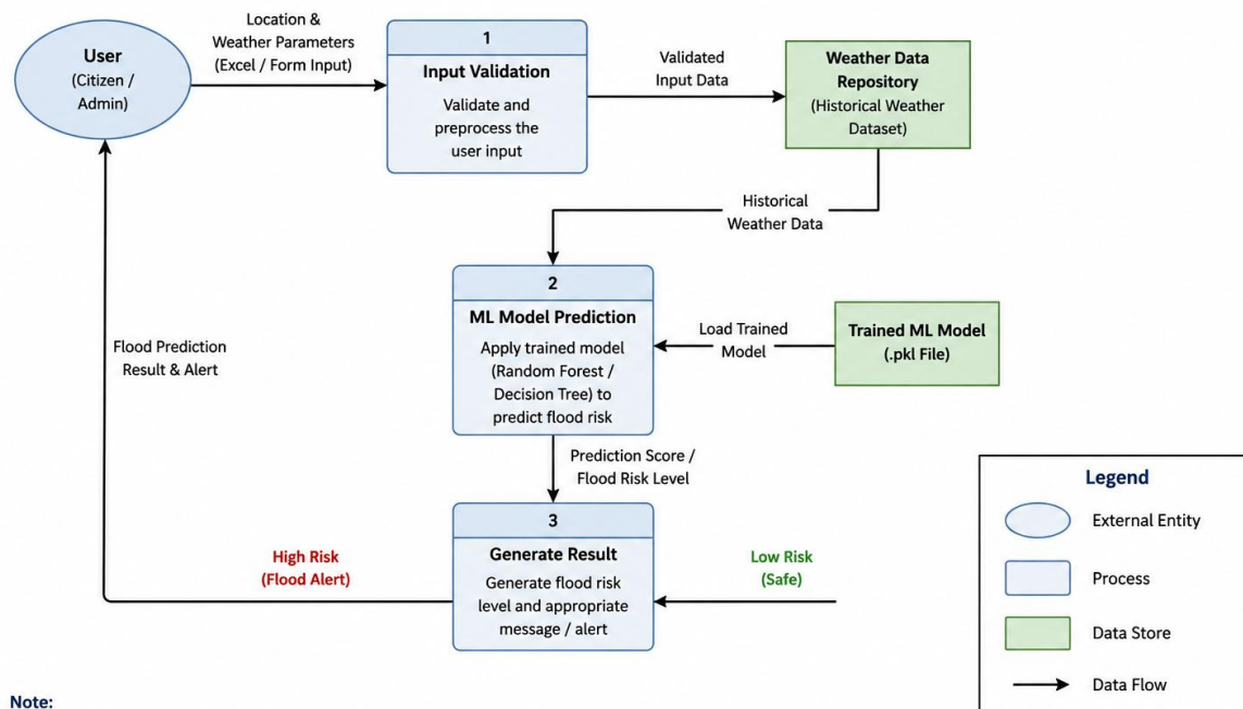
Data Flow Diagram – AIML–RisingWaters (Flood Prediction Using Machine Learning)
